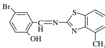
5-Bromosalicylidene-2-amino-4-methylbenzothiazole
