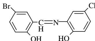
5-Bromosalicylidene-2-amino-4-chlorophenol
