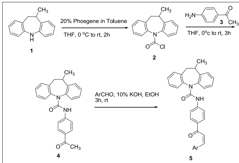
Scheme 1: Synthetic pathway for the compounds 5a-k from 10-methyl-10,11-dihydro-5H-dibenzo[ b,f ]azepine 1
