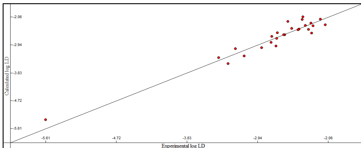
Fig. 1: Comparison of experimental and calculated toxicity of BDZs drugs from the regression analysis in eq. (1). R^2 = 0.932 ; R^2_{cv} = 0.840 ; F=72.20 ; s^2 = 0.077 for 26 BDZs.
