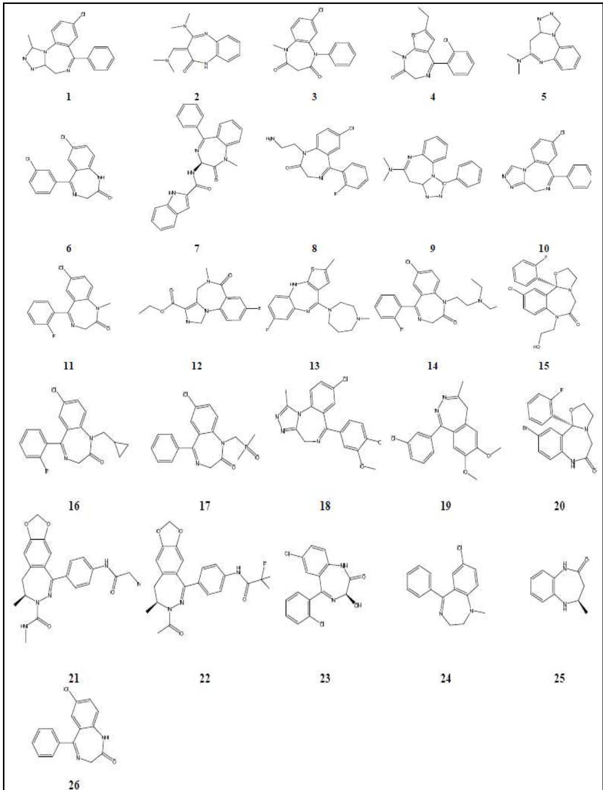
Scheme 1: benzodiazepine drugs (1-26) used in the study
