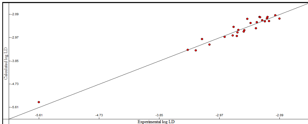
Fig. 2: Comparison of experimental and calculated toxicity of BDZs drugs from the regression analysis in eq. (2). R^2 = 0.959 ; R^2_{cv} = 0.901 ; F=93.87 ; s^2 = 0.024 for 26 BDZs
