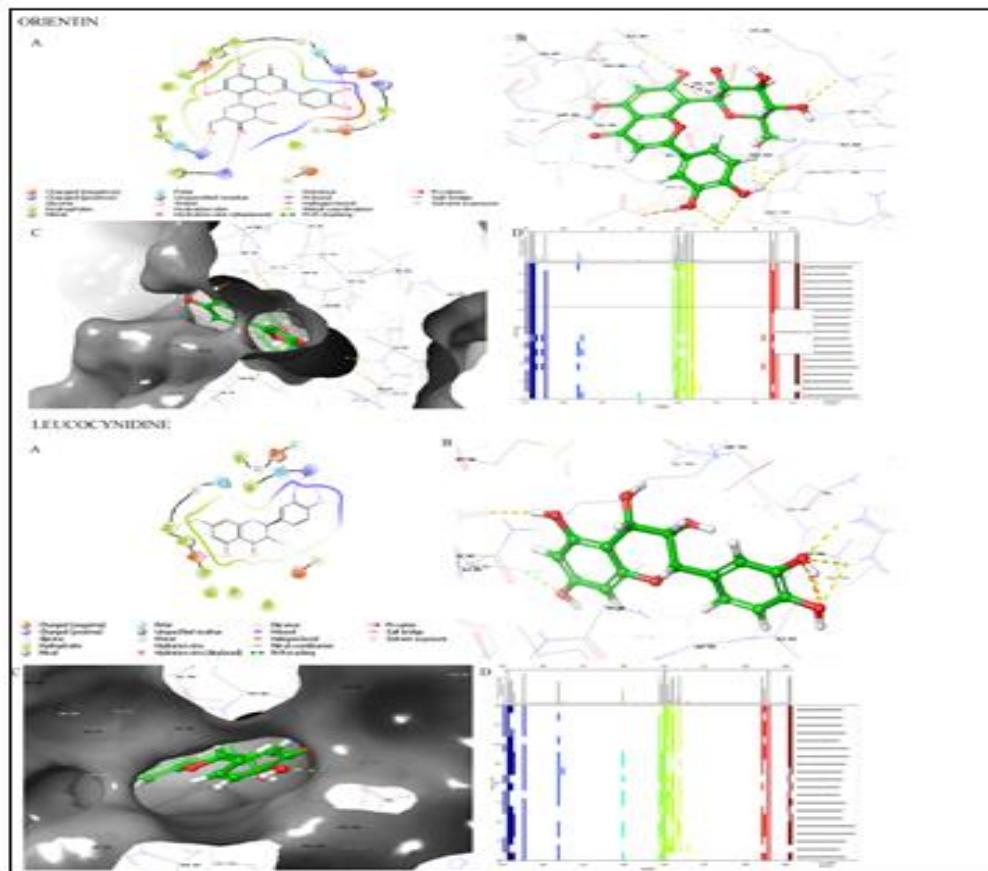
Figure 3: A: 2D Interaction of compound orientin and leucocyanidin with 4K6Z; B: 3D Interaction of compound orientin and leucocyanidin with 4K6Z; C: IFD (surface view) of residues interaction of orientin and leucocyanidin with target protein 4K6Z; D: Fingerprint analysis of IFD.
