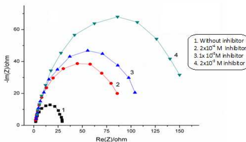
Fig. 3: Nyquist plot for mild steel immersed in 1M H 3 PO 4 containing different concentrations of Bacampicillin
