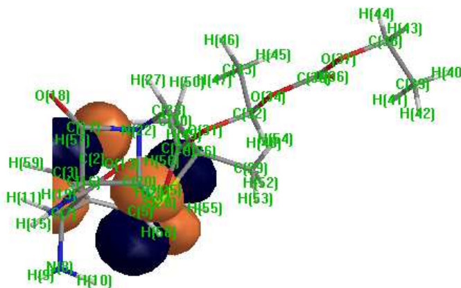
Fig. 9: The lowest unoccupied molecular orbital of Bacampicillin
