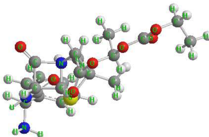
Fig. 7: Optimized structure of Bacampcillin
