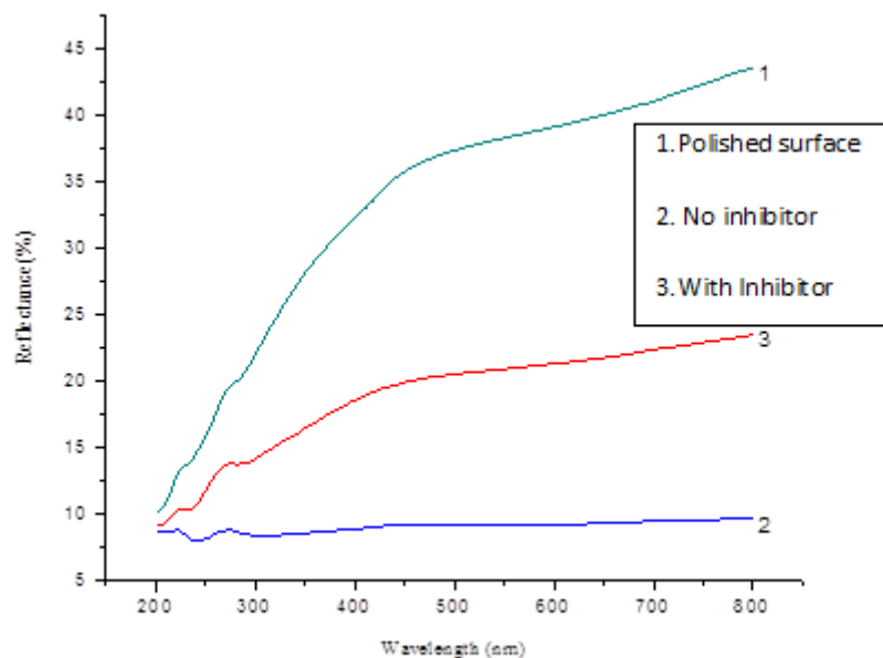
Fig. 4: UV Reflectance curves of mild steel in 1M H 3 PO 4 solution with 20x10 -4 M concentration of the inhibitor
