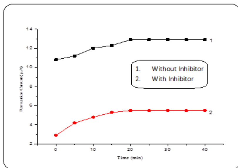
Fig.6: Hydrogen permeation Vs Time curves for mild steel immersed in 1\text{M H}_3\text{PO}_4 and 2 \times 10^{-3}\text{M} concentration of inhibitor
