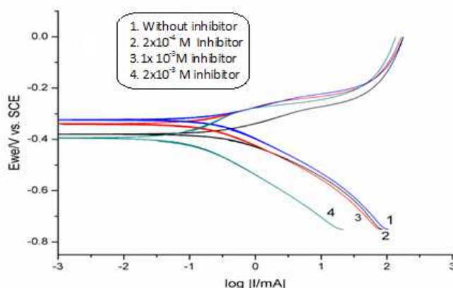
Fig. 2: Polarization curves of mild steel recorded in 1M H_3PO_4 in presence of different concentrations of Bacampicillin
