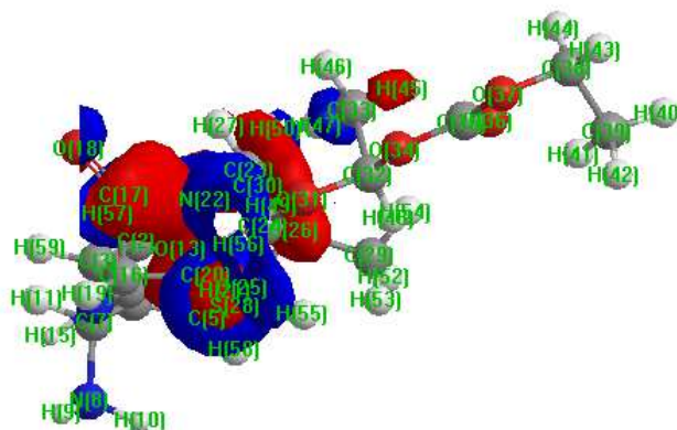
Fig.8: The Highest occupied molecular orbital of Bacampicillin
