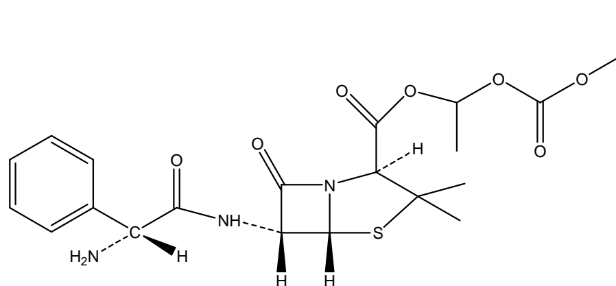
Fig.1: Structure of Bacampicillin
