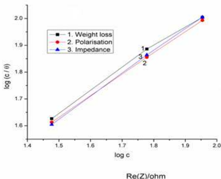
Fig. 5: Langmuir's adsorption isotherm plots for the adsorption Bacampicillin in 1M H 3 PO 4 on the surface of mild steel
