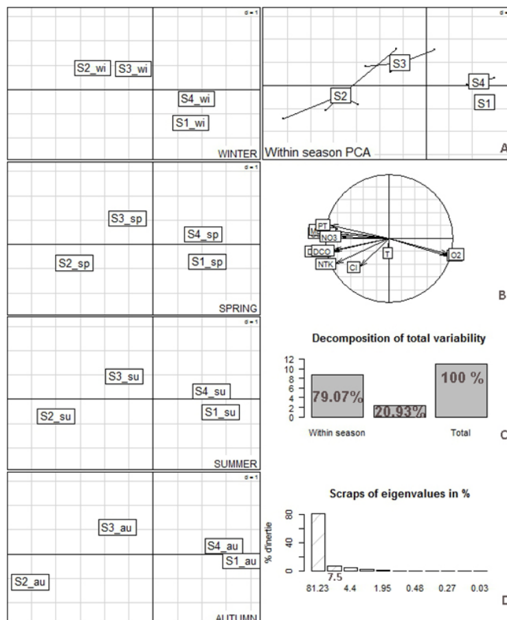
Figure 4: Left top to bottom: graphical representation linking the four factor maps of the intra-season analysis. A: Intra-season PCA; B: Circle of correlations between variables; C: Decomposition of total inertia; D: Eigenvalues histogram of intra-season PCA
