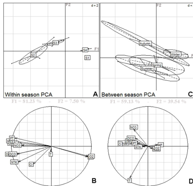
Figure 3: A: Intra-season PCA of 11 environmental variables, B: Intra-season PCA correlation circle, C: Inter-season PCA, D: Inter-season PCA correlation circle
