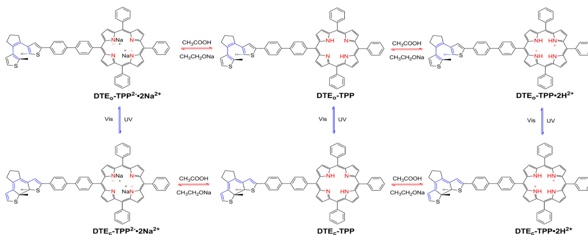
Scheme 2: Schematic of DTE-TPP in alcoholic solution
