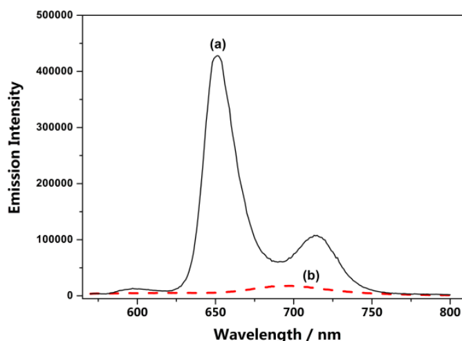
Figure 3: Emission spectra of DTE-TPP in solution of deoxygenated \text{CH}_2\text{Cl}_2 (a) the open form and (b) the closed form. \lambda_{\text{exc}}=530 nm, \lambda_{\text{em}}=651,715 nm
