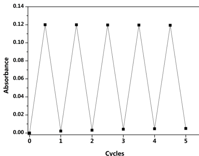
Figure 2: Cycling between the open and closed forms of the DTE-TPP by repetitive irradiation at \lambda=254 nm for 3 min (high value) and visible light for 20 min (low value) at 20^{\circ}\text{C} in \text{CH}_2\text{Cl}_2 . The ordinate shows the formation of the closed form as monitored by the absorbance at 674 nm
