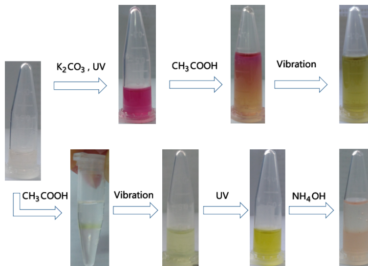
Figure 4: The color changes of the solution of \text{CH}_2\text{Cl}_2 of DTE-TPP
