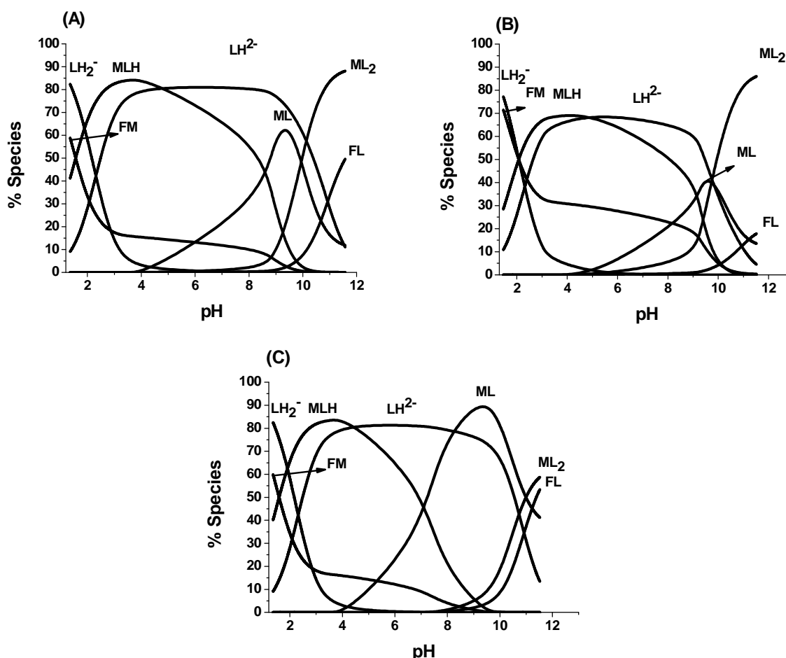
Figure 2: Distribution diagrams of binary complexes of 5-SSA in 10% v/v DMF-water mixture: (a) Co(II), (b) Ni(II) and (c) Cu(II)
