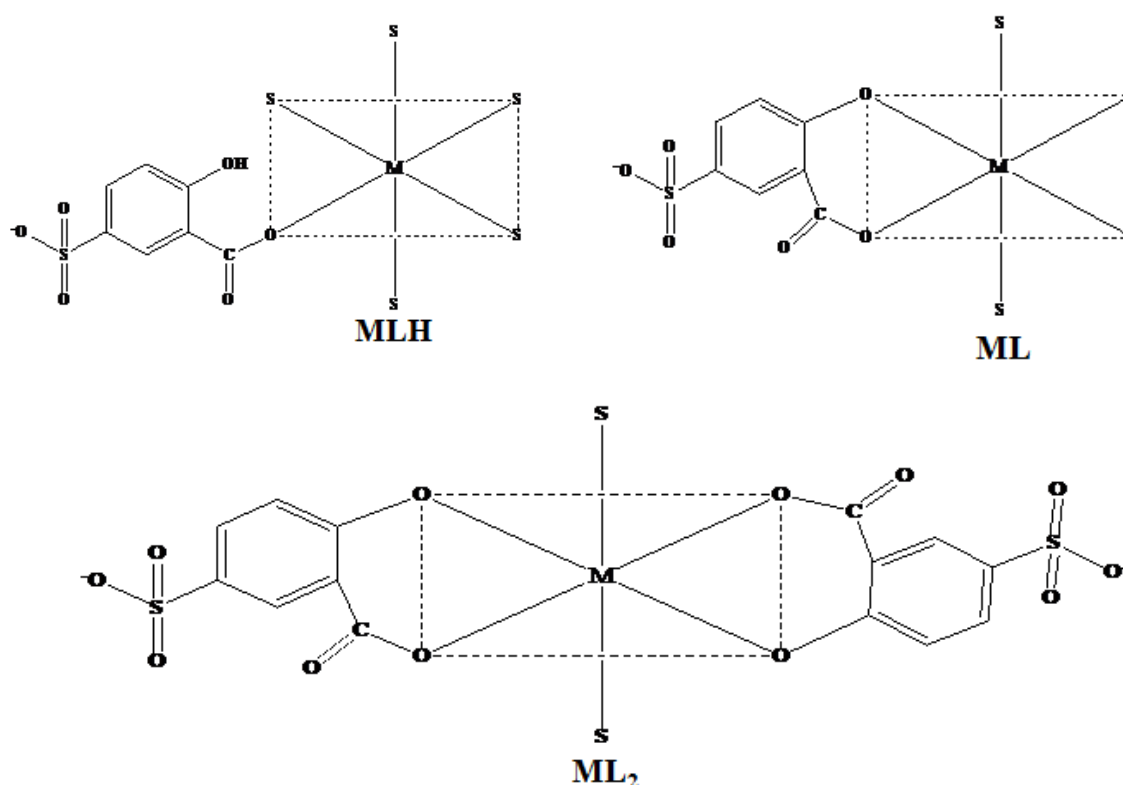
Figure 3: Structure of 5-SSA complexes, where S is either solvent or water molecules
