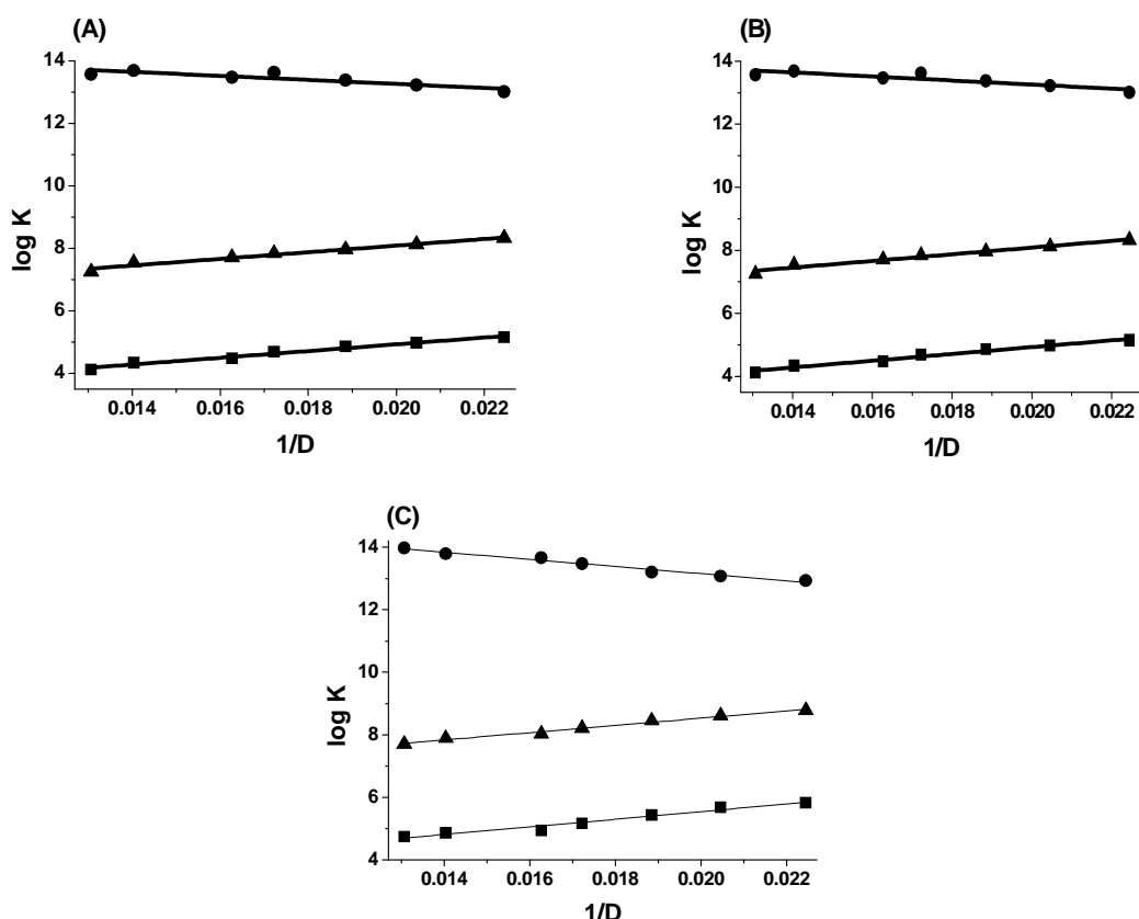
Figure 1. Variation of overall stability constant values of metal-5-SSA complexes with 1/D of DMF-water mixtures (a) Co(II); (b) Ni(II); (c) Cu(II); (■) \log \beta_{ML} ; (●) \log \beta_{MLH} ; (▲) \log \beta_{ML2}
