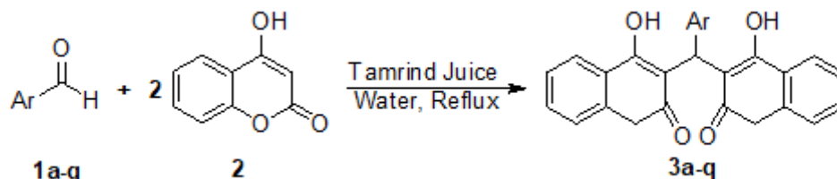
Figure 1: Synthesis of biscoumarin derivatives catalyzed by tamarind juice.
